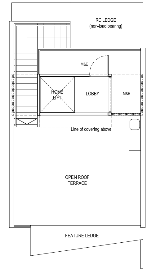
ROOF TERRACE
