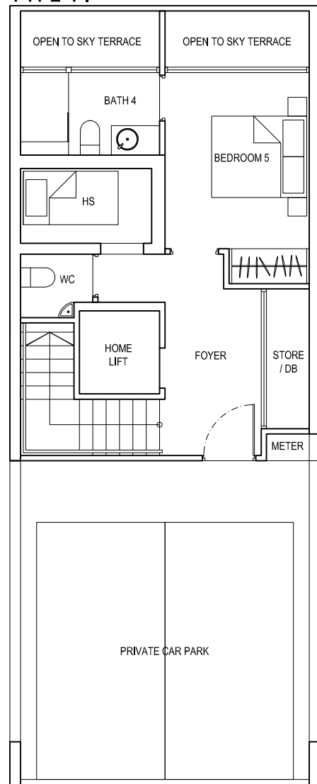
BASEMENT
