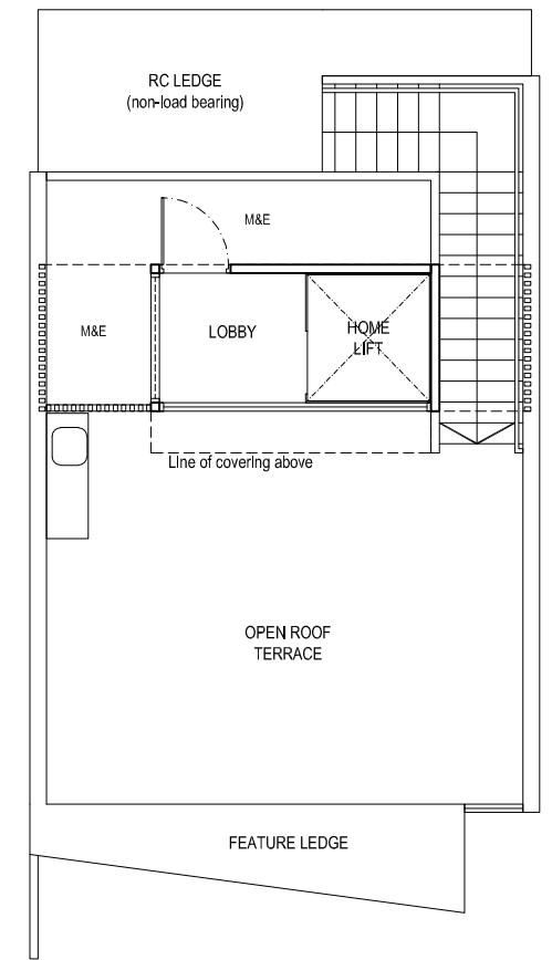
ROOF TERRACE
