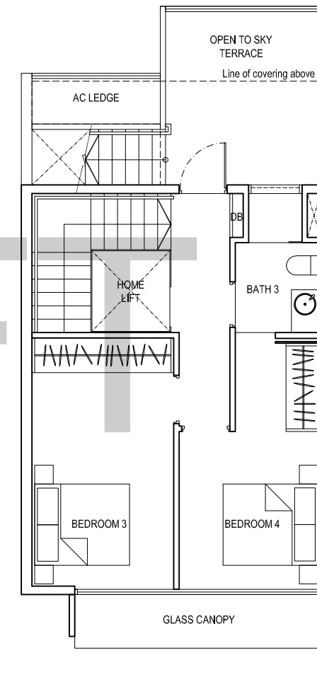
3RD STOREY
