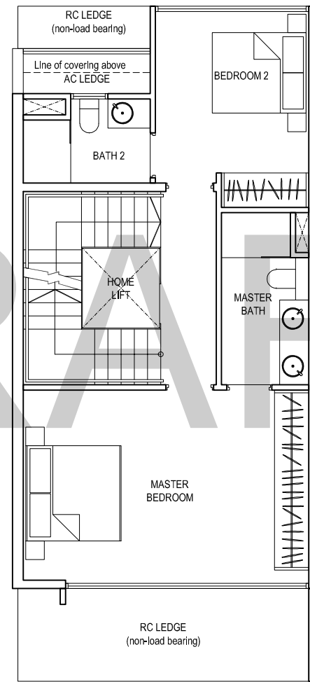
2ND STOREY
